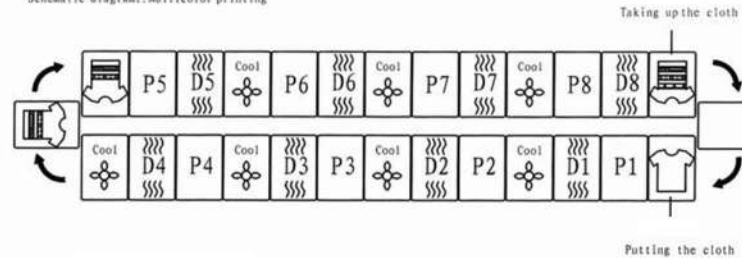
Schematic diagram2: Multicolor production line printing
