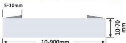
两边压线 Two Edges Sealed
