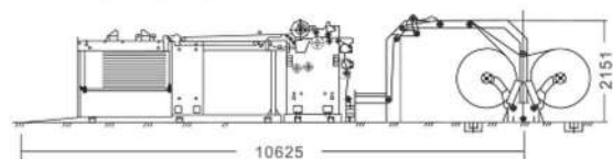
滚刀式切纸机 (二卷) Hob sheet cutting machine (two reel)
