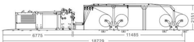
滚刀式切纸机 (四卷) Hob sheet cutting machine (four reel)
