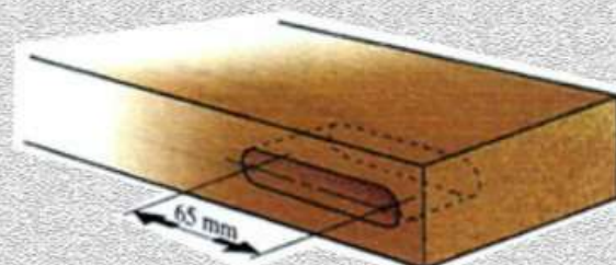
Maximum mortise width-65mm
