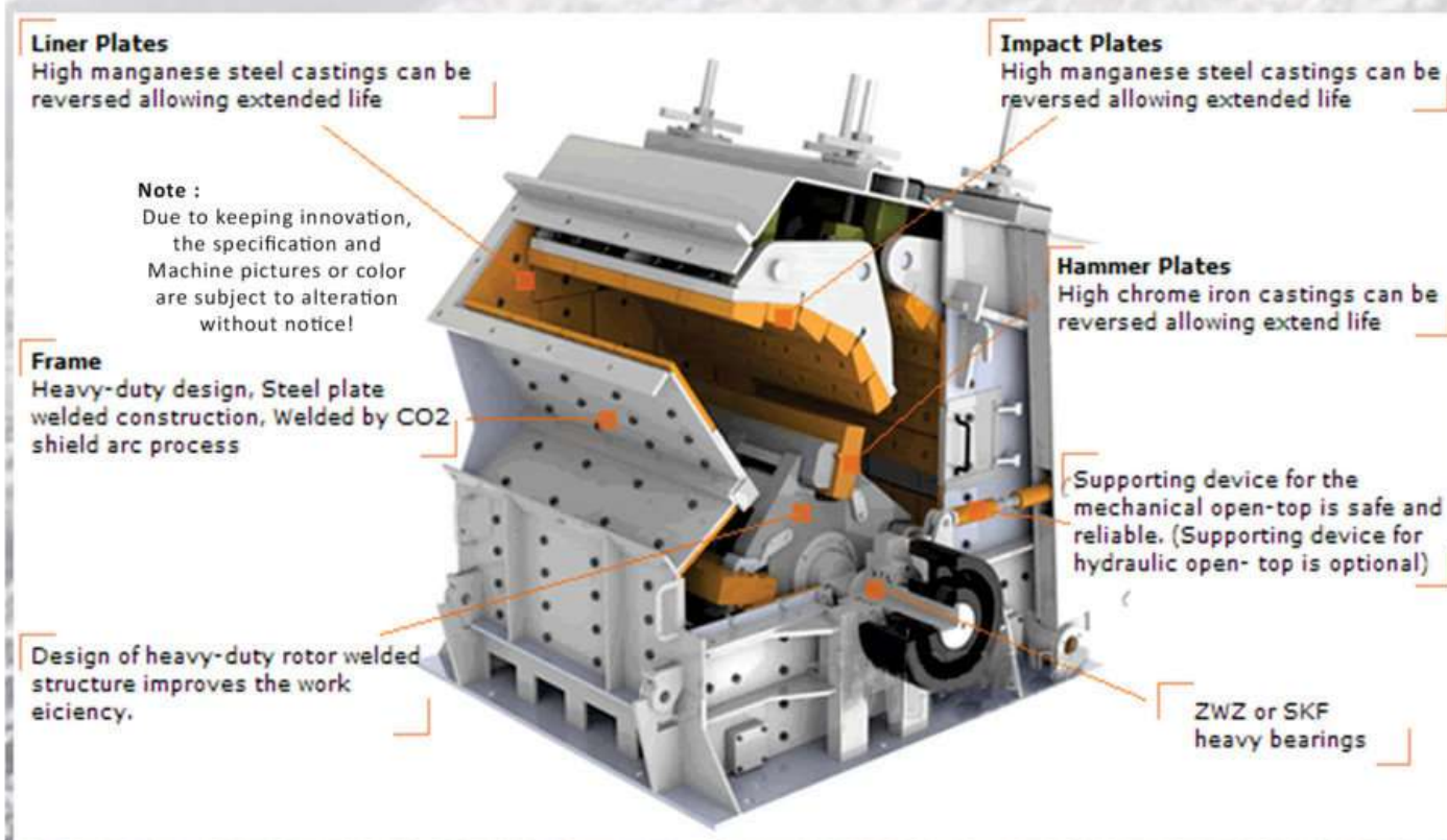
Specification and Technical Parameter of PF Series Impact Crusher
