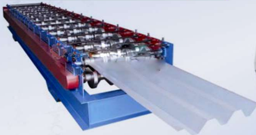
104-520 Dust shield full-automatic roll farming machine
