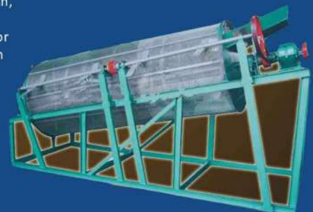
Raw Material Rolling Screen (for hard shale and Coal gangue)
